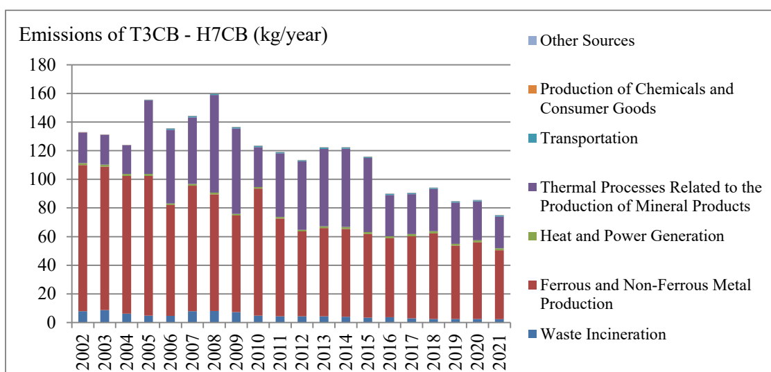
Emission variation of PCB congeners with 3 to 7 chlorine atoms (T3CB-H7CB)
