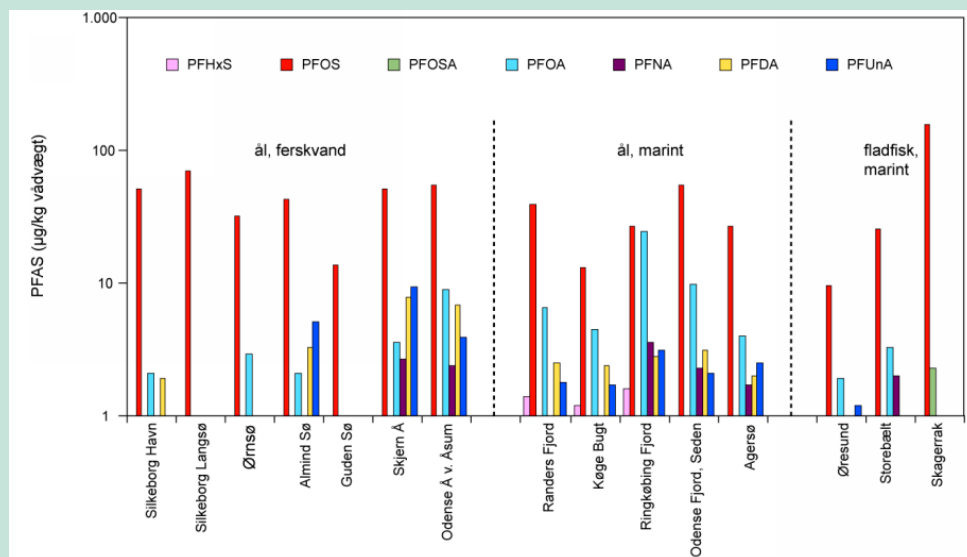
FIGURE 2 MEDIAN CONCENTRATIONS OF PFOS AND OTHER PERFLUORINATED COMPOUNDS IN THE LIVER OF FISH FROM MARINE AND FRESHWATER RECIPIENTS (µG/KG WET WEIGHT) [18]. ÅL, FERSKVAND = EELS, FRESHWATER; ÅL MARINT = EELS, SALTWATER; FLADFISK, MARINT = FLOUNDERS, MARINE
