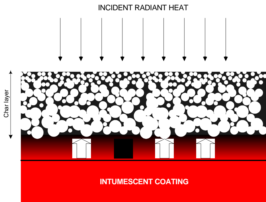
Figure 1 Mechanisms for intumescent systems.
