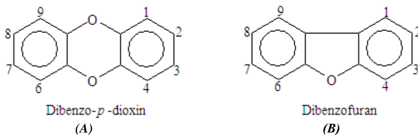
Figure 1: Structures of dibenzo- para -dioxin (A) and dibenzofuran (B)
