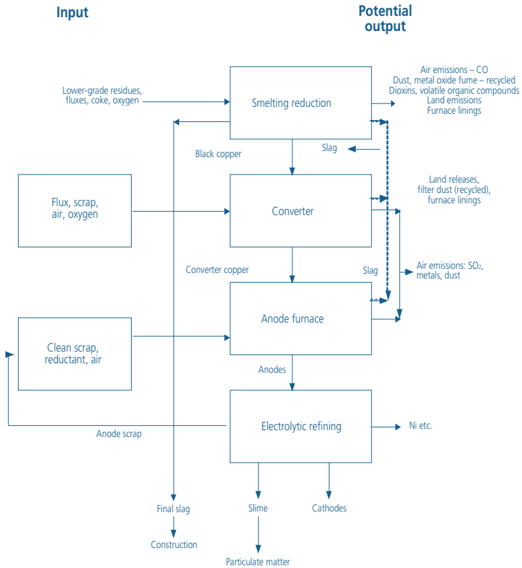
■ Figure 1. Secondary copper smelting
