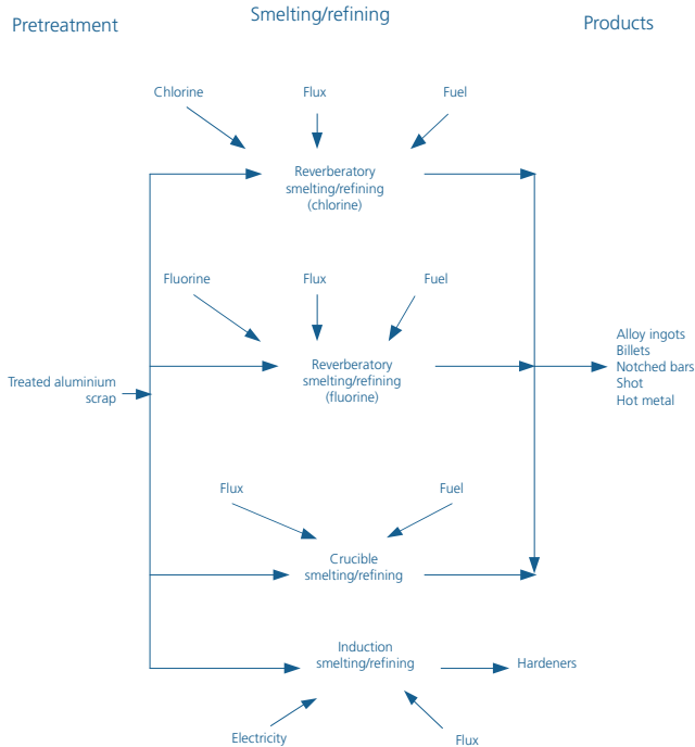
■ Figure 1. Secondary aluminium smelting
