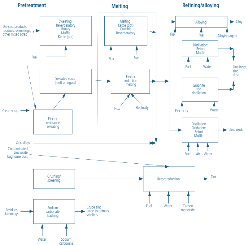
Figure 1. Secondary zinc smelting
