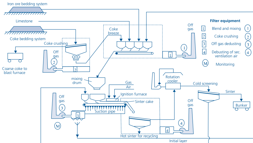
■ Figure 1. Process diagram of a sinter plant
